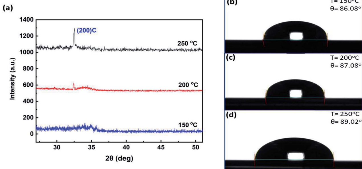
Fig. 3 (a) XRD patterns of ZrO 2 at different temperatures. Measured contact angles on ZrO 2 for 400 cycles at: (b) 150 °C, (c) 200 °C, (d) 250 °C.
