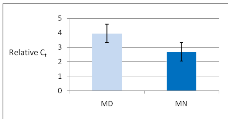
Fig 4. qPCR results indicate that AANAT expression is significantly higher level at midnight (MN) relative to midday (MD). The relative mRNA expression for AANAT gene, was measured using the relative C_t method. Y-axis shows relative C_t values ( C_t of gene of interest – C_t of reference gene). The lower relative C_t value means a higher amount of mRNA. L-24 was used as the reference gene so that the level of melatonin receptor gene expression could be compared between midday and midnight.
