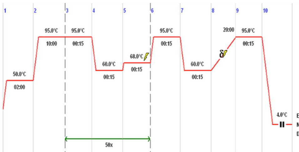
Fig. 1. qPCR was performed according to the temperature template shown above. This figure shows the temperature specifications that were used for qPCR. A total of 50 cycles were run and at the end of each cycle the fluorescence was measured for each sample. Polymerase chain reaction was done in two main steps: holding the reagents at 95°C for 15 sec (denaturation) followed by at 60°C for 15 sec and 68°C for 15 sec (annealing and extension). Step 8 shows the melting curve analysis, where temperature is increasing from 60°C to 95°C with a continuous measuring of fluorescence.
