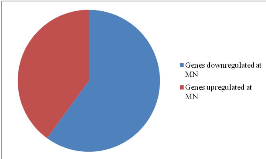
Fig.2. A total 44 genes showed significant change of 2-fold or more. At midnight there were 26 genes that showed decreased expression and 18 genes that showed increased expression as compared to midday.
