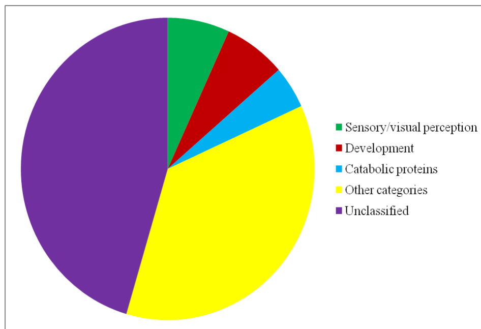
Figure 3. Analysis of gene ontology for 44 genes according to biological function.
